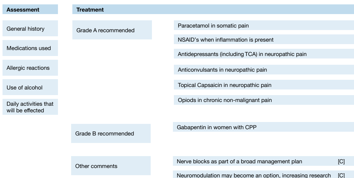
Figure 18: algorithm for the use of neuropathic analgesics
