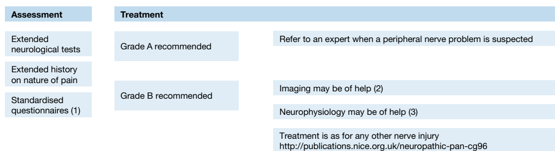
Figure 14: assessment and treatment algorithm for peripheral nerve pain syndrome
